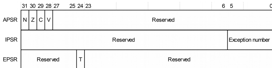
Figure 24-3. PSR
