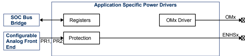
Figure 23-1. Application Specific Power Driver
