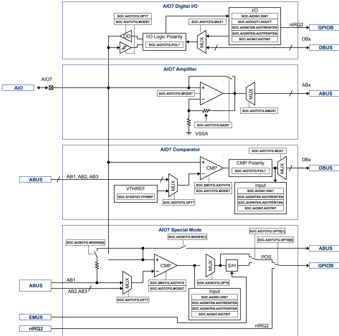
Figure 22-6. AIO7
