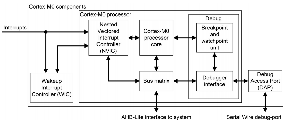
Figure 24-1. Cortex-M0 implementation
