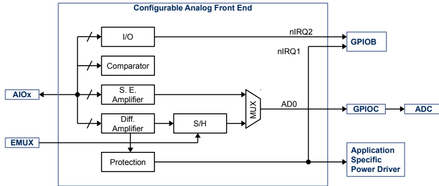
Figure 22-1. Configurable Analog Front End
