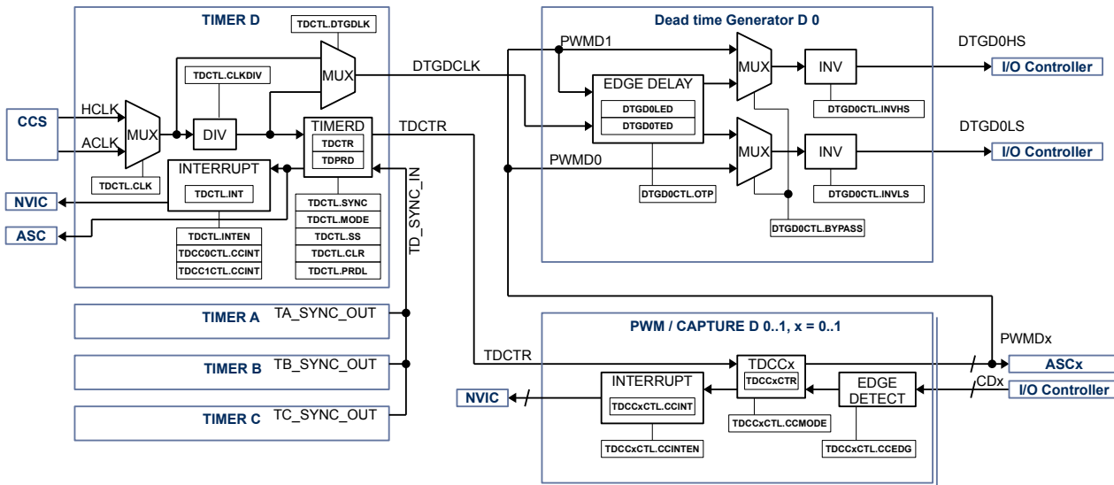
Figure 14-1. Timer D
