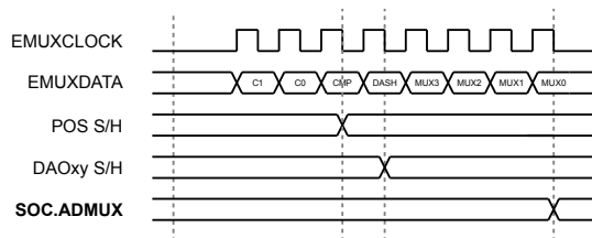
Figure 22-10. EMUX Timing
