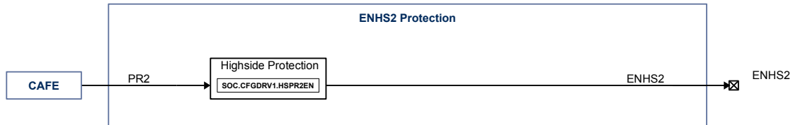
Figure 23-6. ENHS2 Protection
