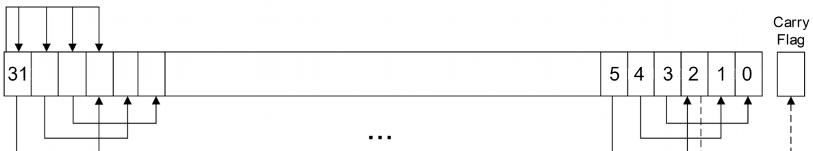
Figure 24-11. ASR #3
