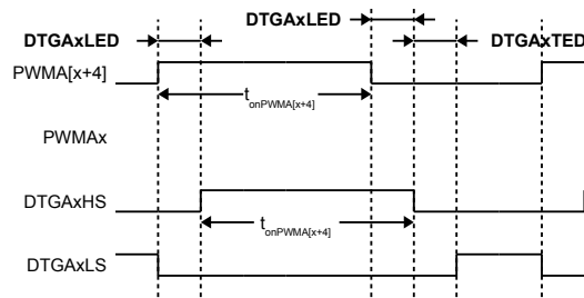
Figure 11-7. DTGx LED and TED with On Time Preservation Example
