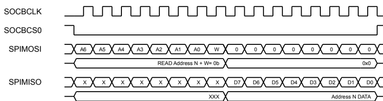
Figure 19-2. Single Read from SOC Bridge
