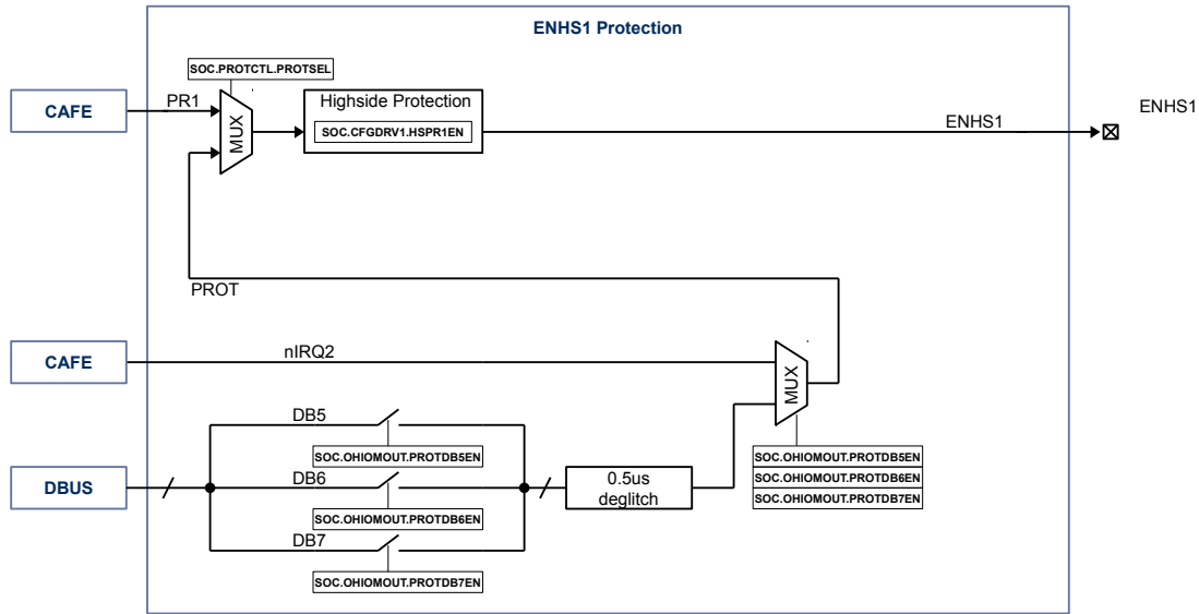
Figure 23-5. ENHS1 Protection
