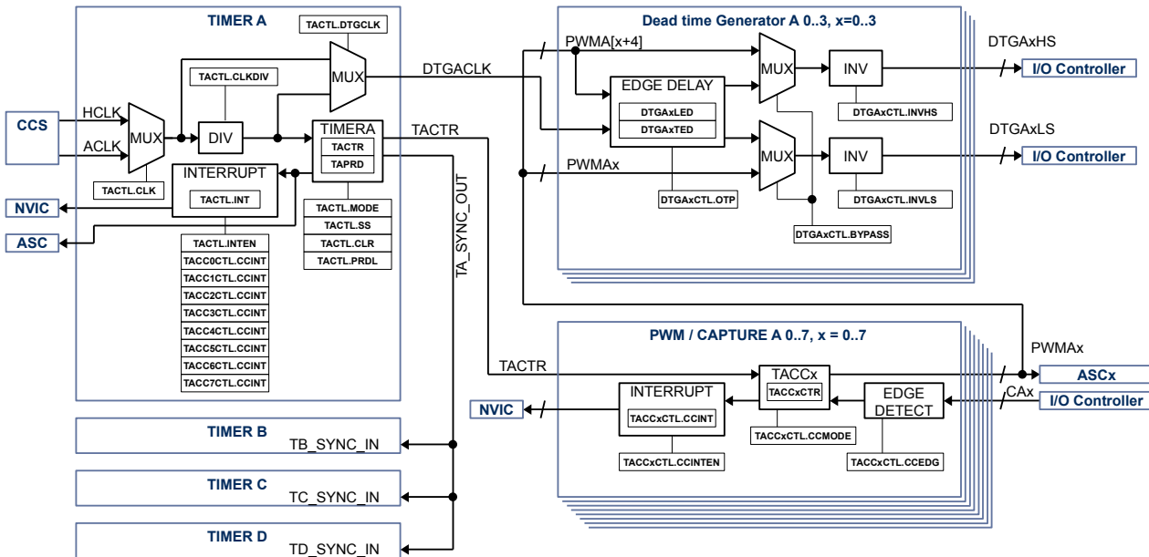
Figure 11-1. Timer A
