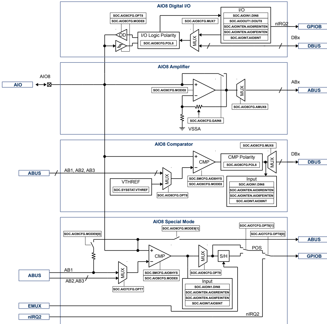
Figure 22-7. AIO8
