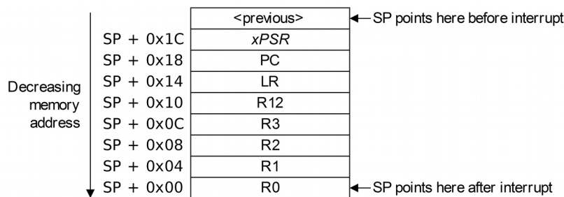
Figure 24-10. Exception Entry Stack Contents
