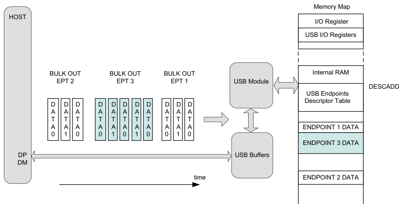
Figure 30-4. OUT Transfer: Data Packet Host to USB Device
