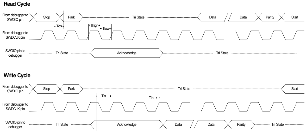
Figure 35-15. SWD Interface Signals
