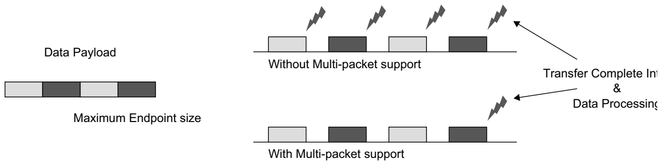
Figure 30-3. Multi-Packet Feature - Reduction of CPU Overhead
