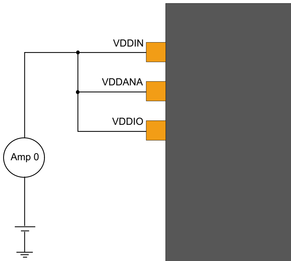
Figure 35-1. Measurement Schematic
